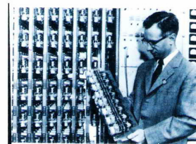
Fig. 1.5. • Charles Wightman holding a subrack of 8 motor/potentiometer pairs. Each potentiometer pair functioned as a single adaptive weight value. The perceptron 8 law was implemented in analog circuits that when properly wired through the board shown in Figure 1.6, would control the motor of each potentiometer (the one of which functioned to implement one weight). Photo courtesy of Arvin Calspan Advanced Technology Center.
