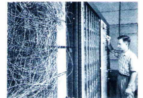
Fig. 1.6. • The Mark I Perceptron patchboard. The connection patterns were typically "random", so as to illustrate the ability of the perceptron to learn the desired pattern without need for precise wiring (in contrast to unlike the precise wiring required in a programmed computer). Photo courtesy of Arvin Calspan Advanced Technology Center.
